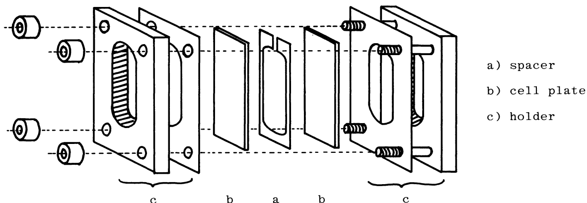
Fig. 1. Vessel for restricted reaction.
